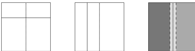
Figure 10.5: Left: [0, 1]^2 with the line x = 1/2 marked dotted and \int_0^1 f(x, y) dx marked as a gray solid line for a generic y . Center: Similar picture but \int_0^1 f(x, y) dy marked for some x \neq 1/2 . Right: The three different rectangles in the partition used to integrate f in different grays.
