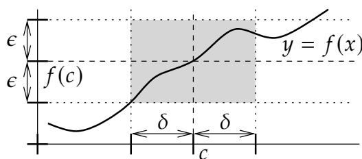
Figure 3.3: For |x - c| < \delta , the graph of f(x) should be within the gray region.
