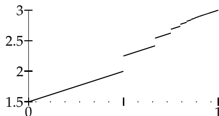
Figure 3.12: Strictly increasing function on [0, 1] with countably many discontinuities.
