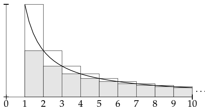
Figure 5.10: The area under the curve, \int_1^\infty f , is bounded below by the area of the shaded rectangles, f(2) + f(3) + f(4) + \cdots , and bounded above by the area of the entire rectangles, both the shaded and unshaded parts, f(1) + f(2) + f(3) + \cdots .
