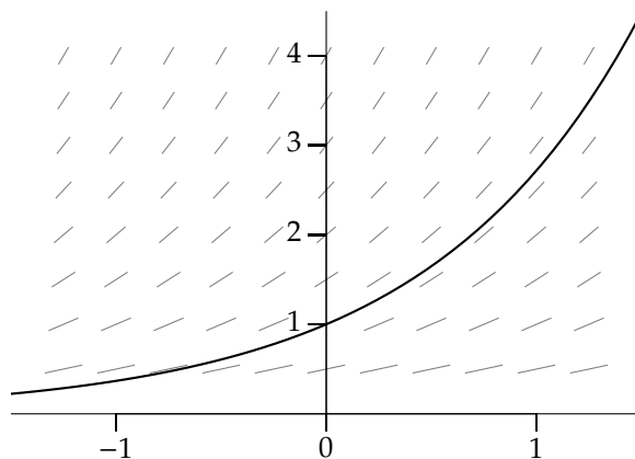
Figure 5.7: Plot of e^x , together with a slope field giving slope y at every point (x, y) . The equation \frac{d}{dx}e^x = e^x means that y = e^x follows these slopes.
