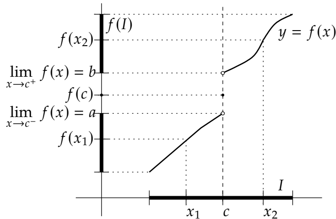
Figure 3.11: Increasing function f: I \rightarrow \mathbb{R} discontinuity at c .
