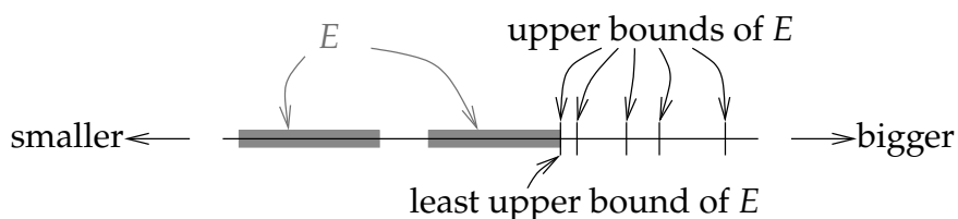
Figure 1.1: A set E bounded above and the least upper bound of E .
