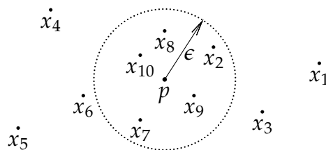
Figure 7.10: Sequence converging to p . The first 10 points are shown and M = 7 for this \epsilon .
